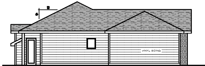
LEFT ELEVATION
